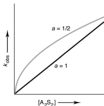
Figure 4. Plot of k_{\text{obs}} versus LDA concentration ( [A_2S_2] ) showing the reaction orders in LDA ( a ).
