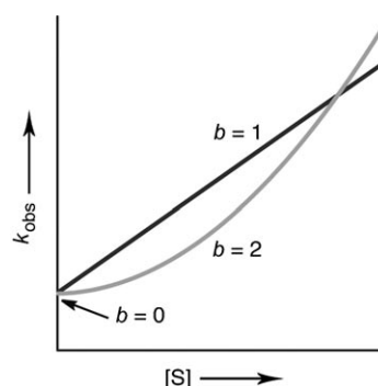
Figure 6. Plot of k_{\text{obs}} versus solvent concentration ( [S] ) showing solvent orders ( b ) for parallel reaction pathways.
